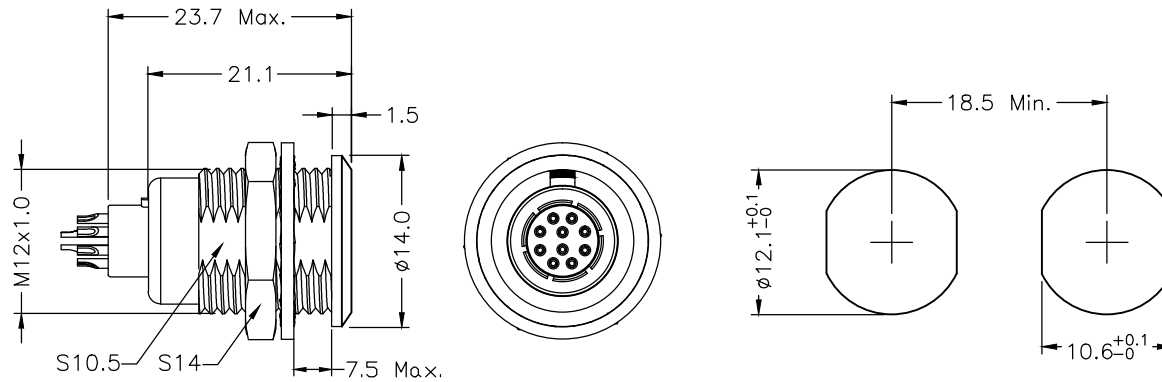
PANEL CUT-OUT
